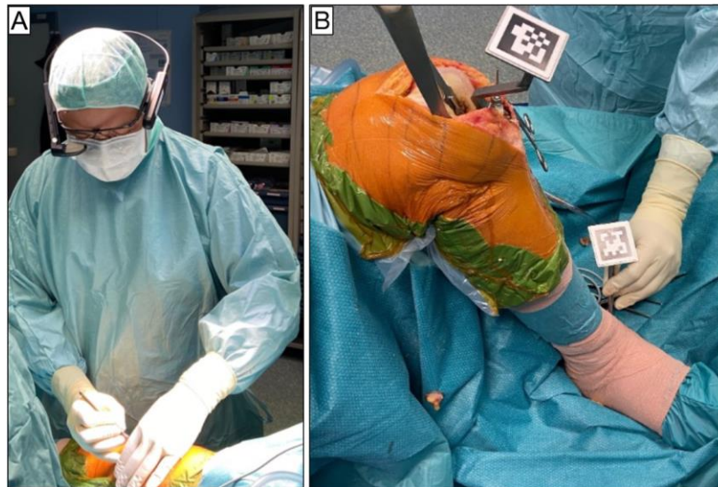
A: Vuzix Smart Glasses worn by the surgeon during surgery. B: The surgeon registers bone landmarks consisting of lateral and medial malleolus using the pointer with QR-Codes.
